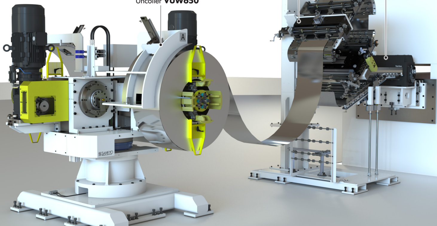
Uncoiler VUW650
